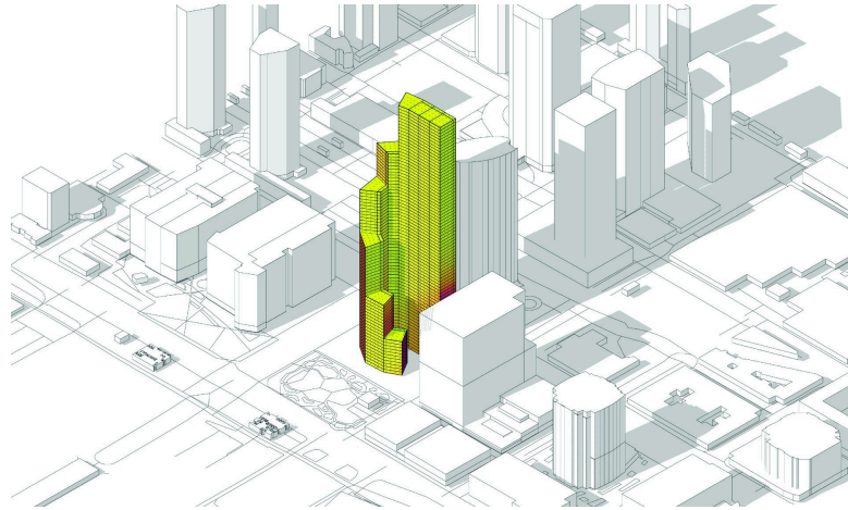
OVERHANG DEPTH STUDIES: MAX DEPTH EXAGGERATED SO THE CHANGE IS VISIBLE
