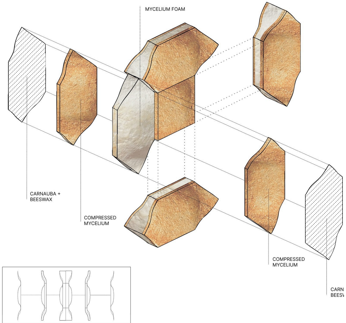
MULTI-DENSITY MYCO-BLOCK: COMPRESSED MYCELIUM SKIN AROUND A FOAM CORE, WITH A CARNAUBA AND BEESWAX COATING
