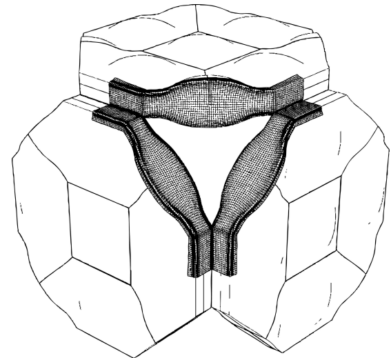
CORNER JOINT DETAIL
